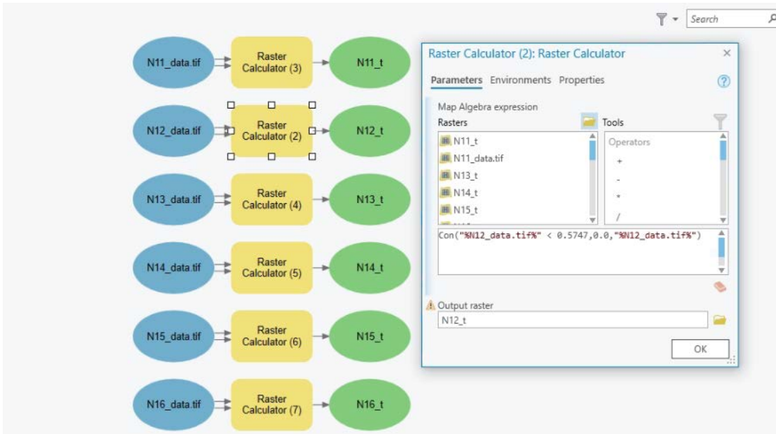
Figure 5.2 Model 1. ARCGIS PRO graphical model for thresholding each habitat suitability map
